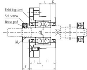
View X-X (example 1)
